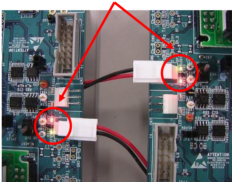
図 9.3-9 CAN 通信成功時の LED
