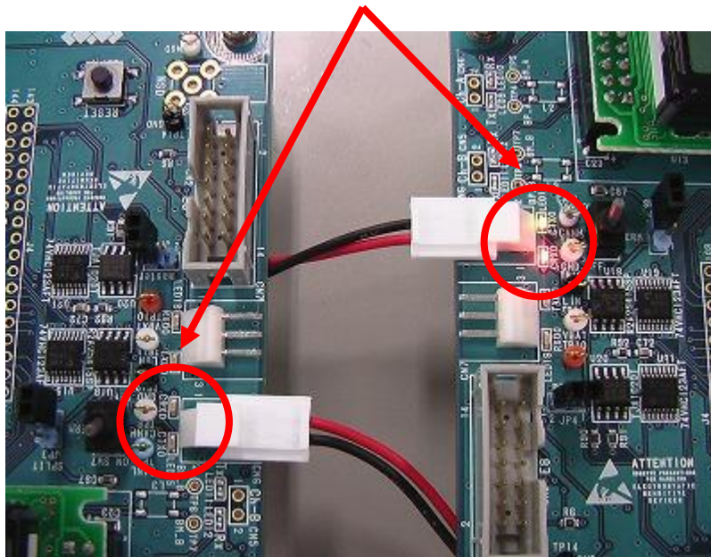
図 9.3-10 CAN 通信失敗時の LED
